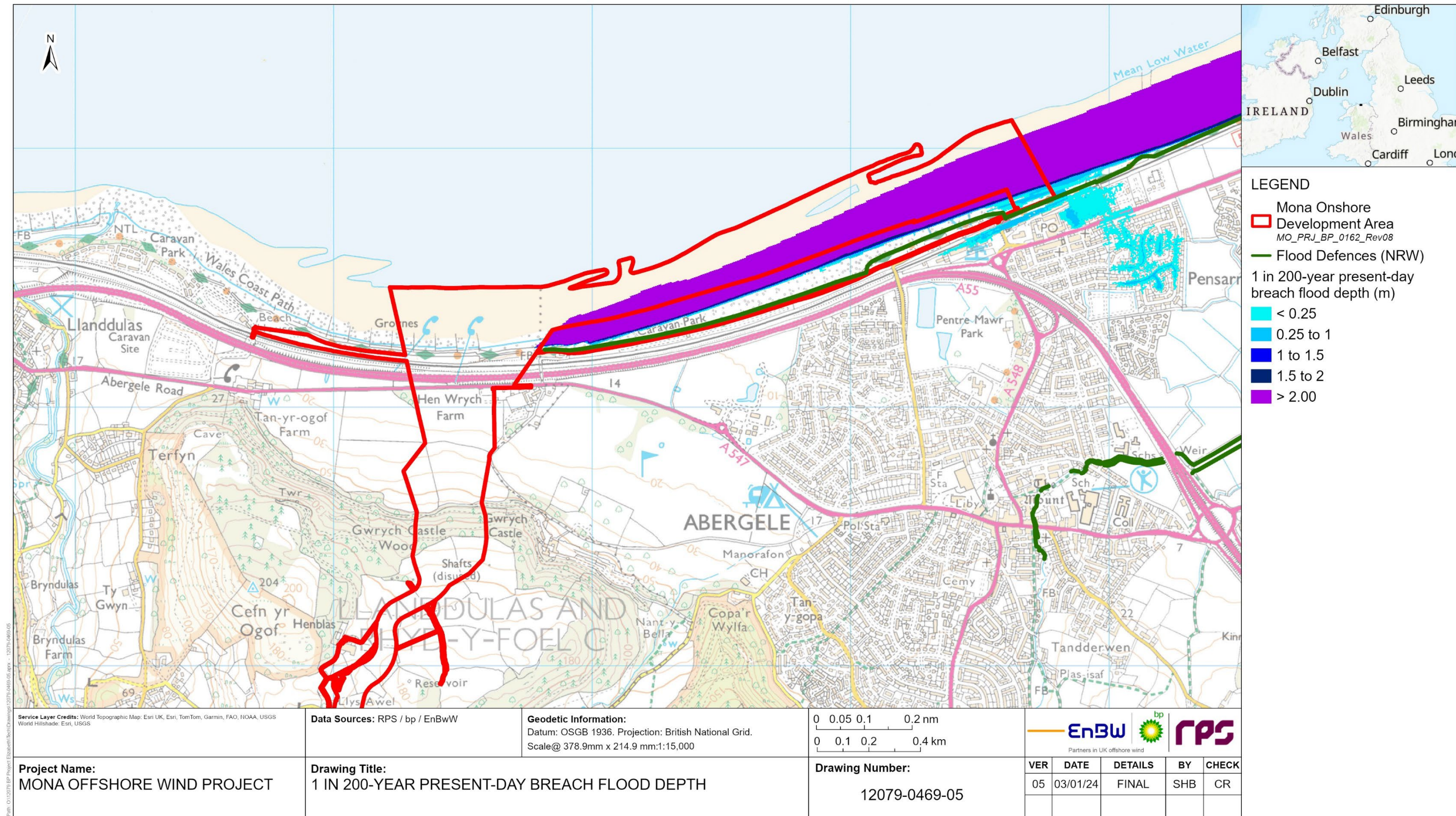
Figure 1.9: 1 in 200-year present day tidal breach flood map.
